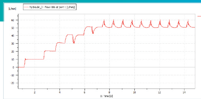
Flowrate through the filling machine.
