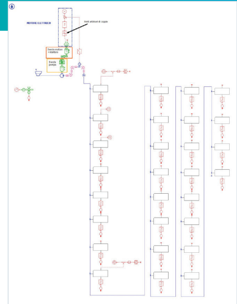
Complete filling-machine system modeled with Simcenter Amesim.
